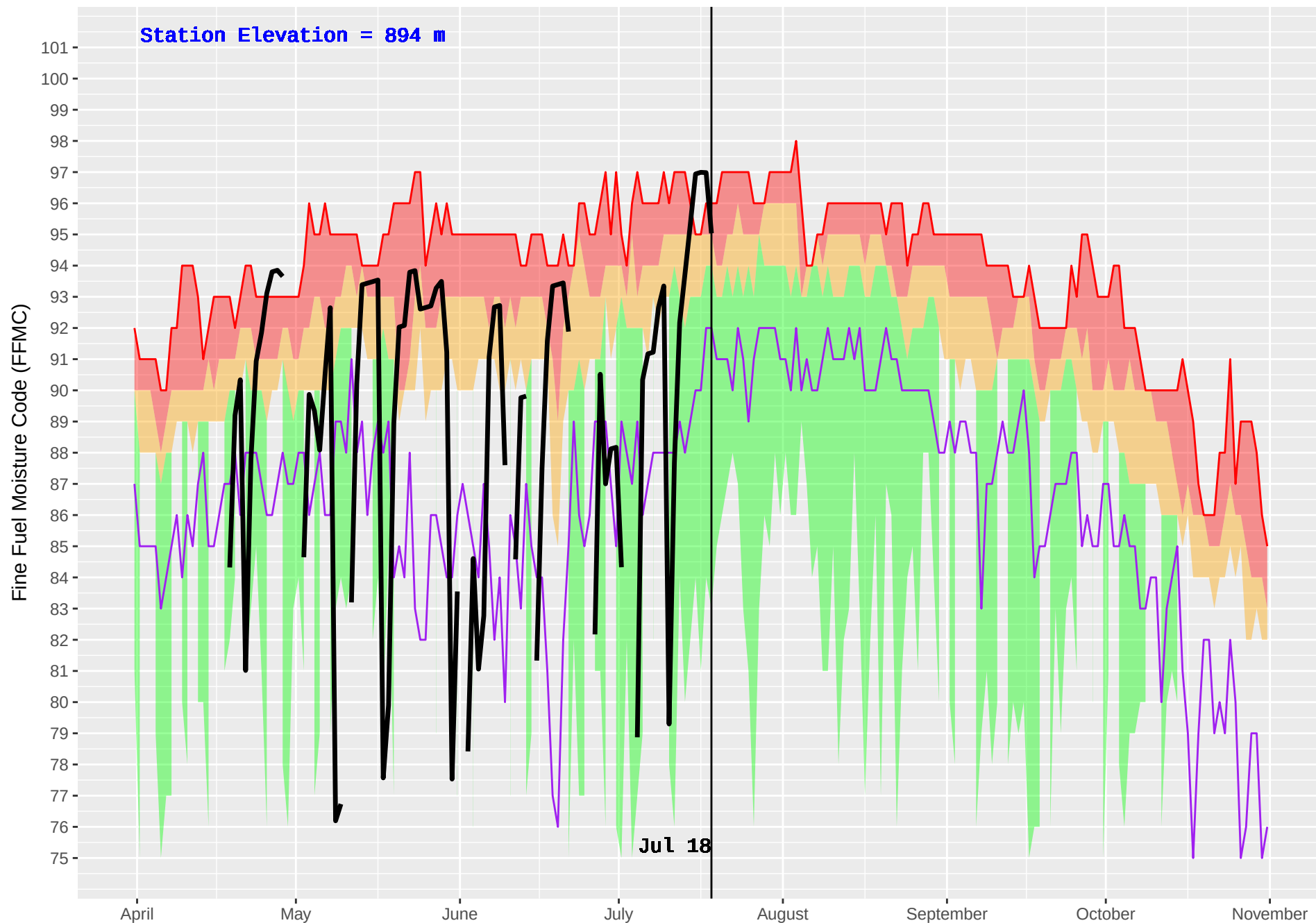
TOBY HUB (417) : Historical (1986–2016) and Current (2018) Daily Fine Fuel Moisture Code (FFMC)
